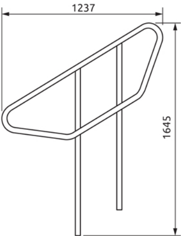
ED-SHR-SBA-S1 weight: 7kg, material: steel tube Ø 35 x 1,5mm finish: galvanized, option - powder coating
