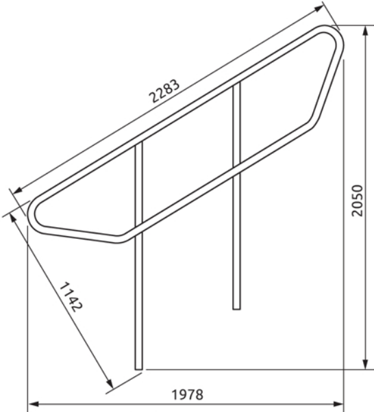
ED-SHR-SBA-S2 weight: 9kg, material: steel tube Ø 35 x 1,5mm finish: galvanized, option - powder coating
